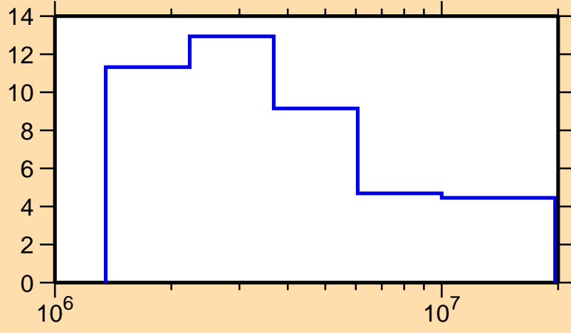
\Delta\sigma/\sigma vs. E for ^{167}\text{Ho}(n,n\text{onel.})
