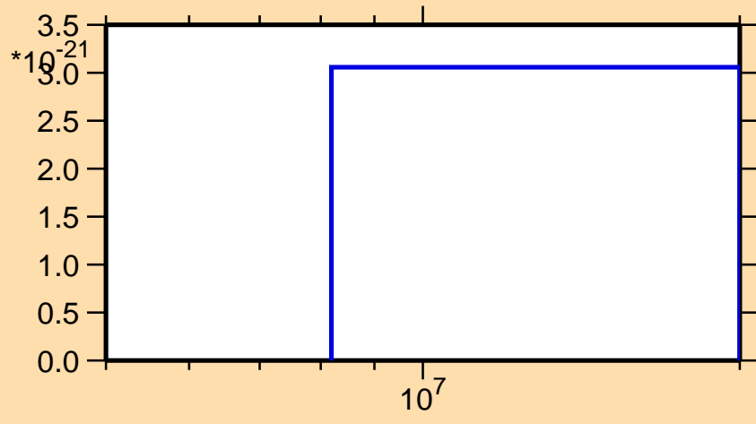
\sigma vs. E for ^{167}\text{Ho} (mt 42)
