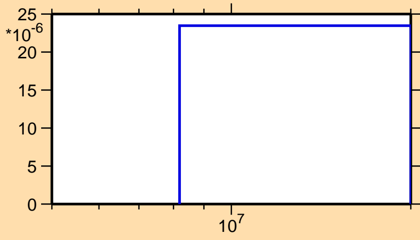
\sigma vs. E for ^{167}\text{Ho}(n,t)
