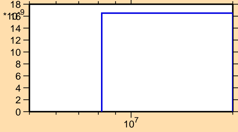
\sigma vs. E for ^{167}\text{Ho}(n,nt)
