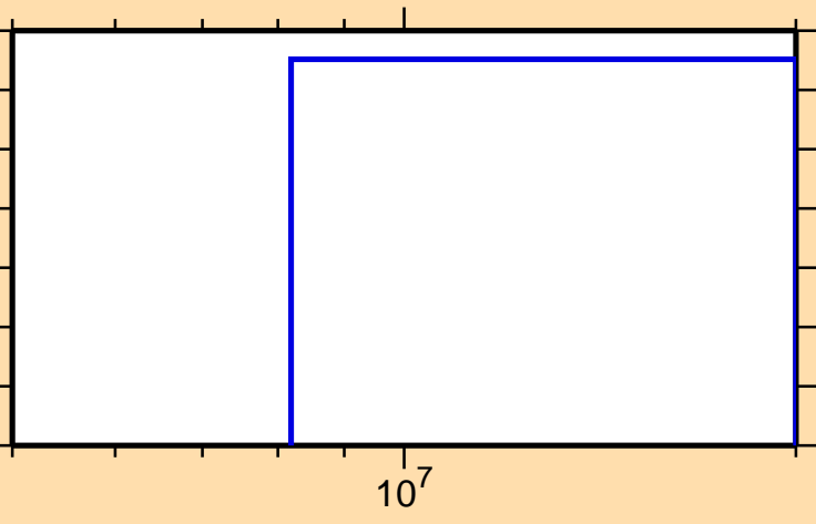
\sigma vs. E for ^{167}\text{Ho}(n,\text{nd})
