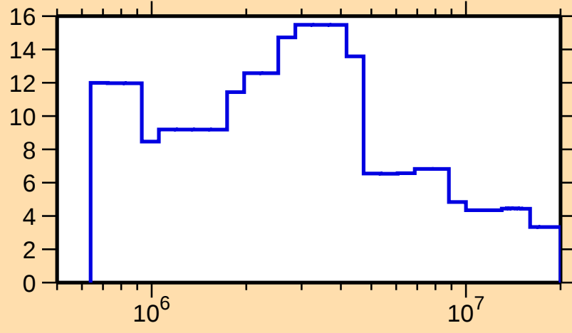
\Delta\sigma/\sigma vs. E for ^{168}\text{Ho}(n,n\text{nonel.})
