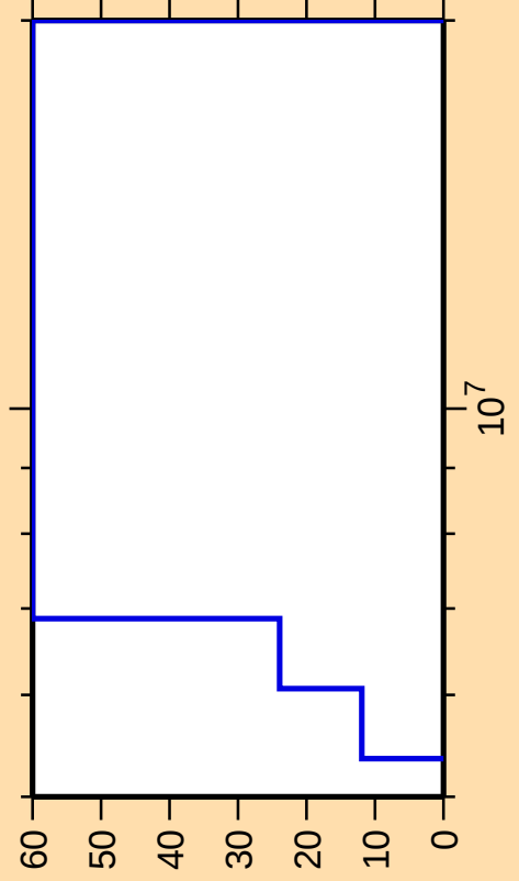
\Delta\sigma/\sigma vs. E for ^{168}\text{Ho}(n,n\text{cont.})
