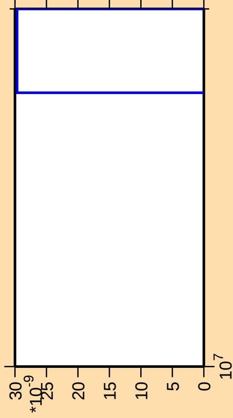
\Delta\sigma/\sigma vs. E for ^{168}\text{Ho} (mt 42)
