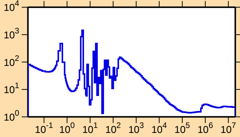
\sigma vs. E for ^{168}\text{Ho}(n,\text{nonel.})
