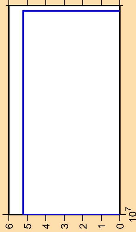
\Delta\sigma/\sigma vs. E for ^{169}\text{Ho}(n,3n)
