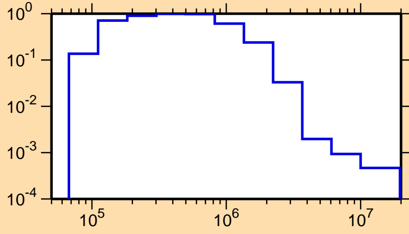
\sigma vs. E for ^{169}\text{Ho}(n,n_1)
