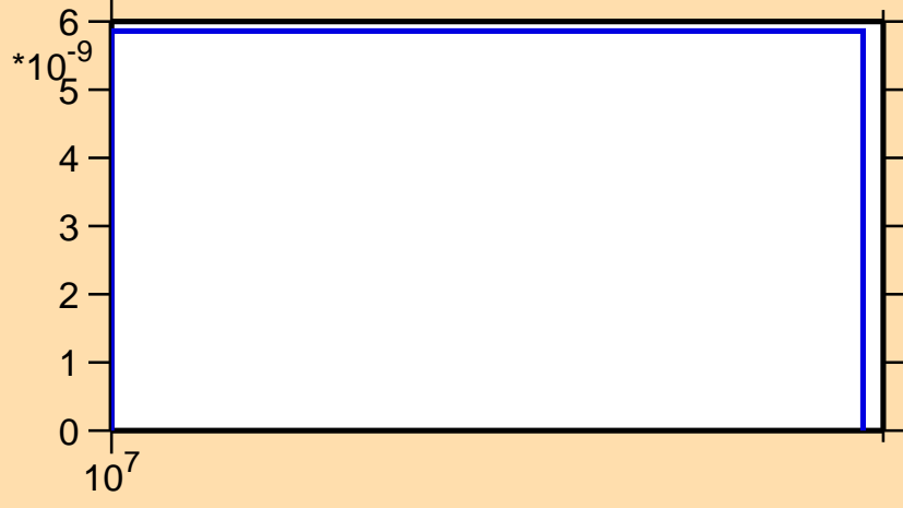
\sigma vs. E for ^{169}\text{Ho}(n,\text{nd})
