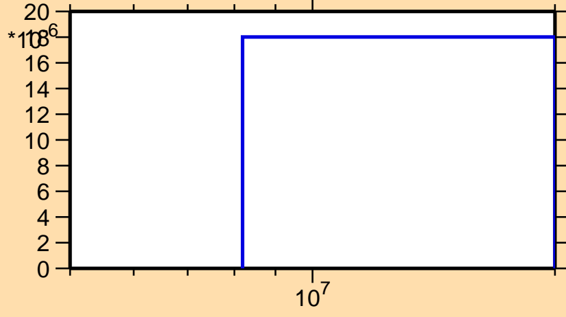
\sigma vs. E for ^{169}\text{Ho}(n,t)
