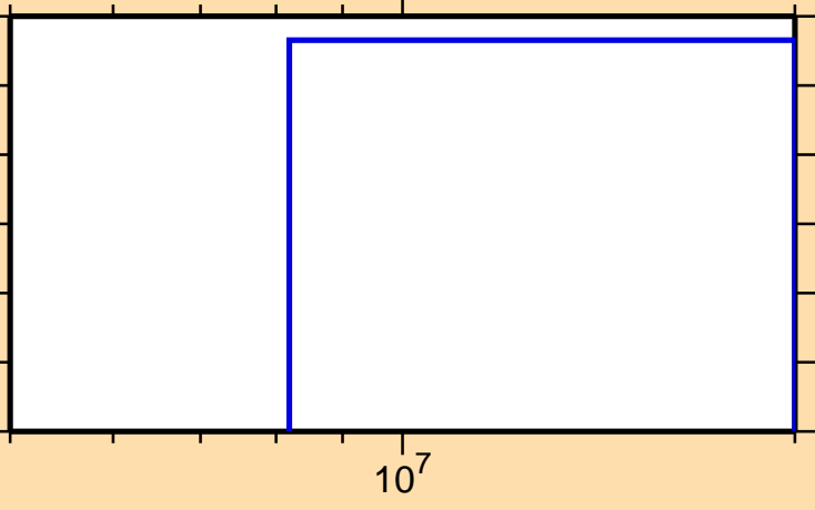
\sigma vs. E for ^{169}\text{Ho}(n,\text{nd})
