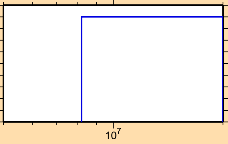
\sigma vs. E for ^{169}\text{Ho}(n,t)
