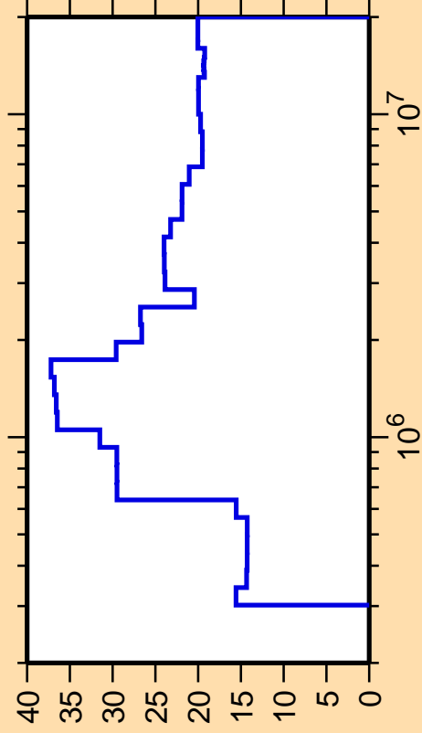
\Delta\sigma/\sigma vs. E for ^{170}\text{Ho}(n,n_2)
