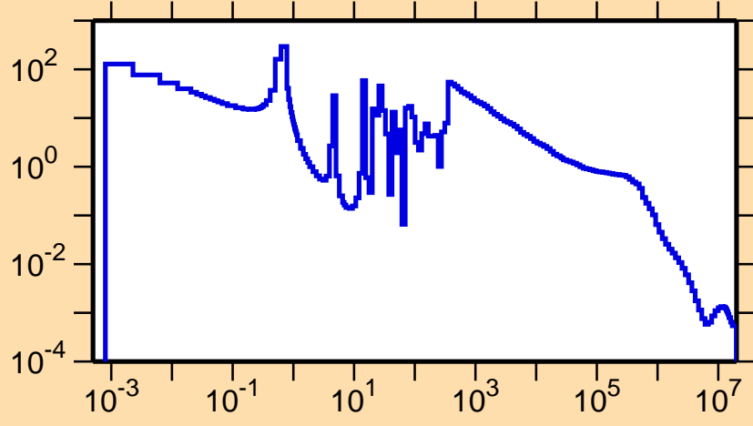
\sigma vs. E for ^{170}\text{Ho}(n,\gamma)
