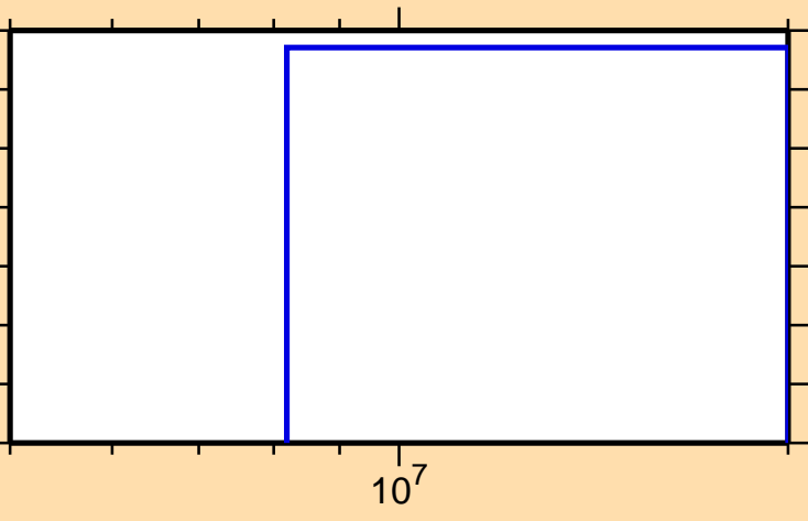
\sigma vs. E for ^{170}\text{Ho}(n,\text{He3})
