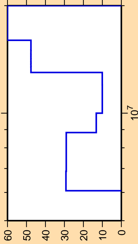
\Delta\sigma/\sigma vs. E for ^{171}\text{Ho}(n,2n)
