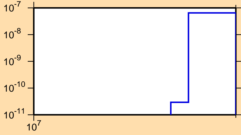
\sigma vs. E for ^{171}\text{Ho}(n,2np)
