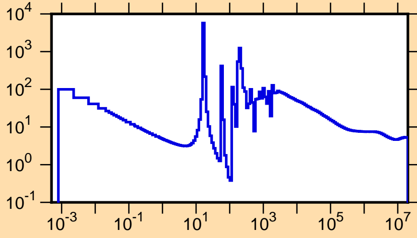
\sigma vs. E for ^{171}\text{Ho}(n,\text{tot.})
