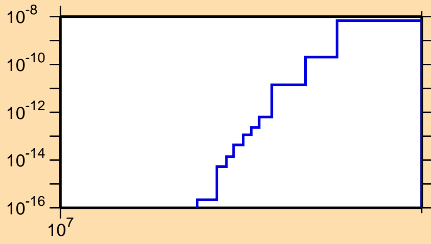
\sigma vs. E for ^{171}\text{Ho}(n,2n\alpha)
