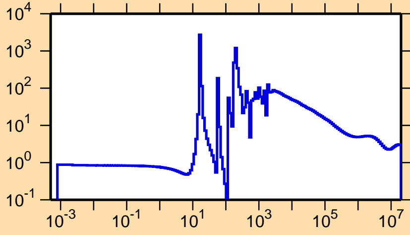
\sigma vs. E for ^{171}\text{Ho}(n,\text{el.})
