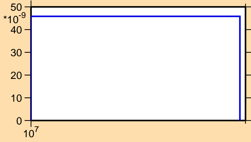
\sigma vs. E for ^{171}\text{Ho}(n,nt)
