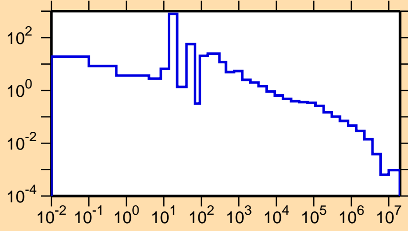
\sigma vs. E for ^{171}\text{Ho}(n,\gamma)
