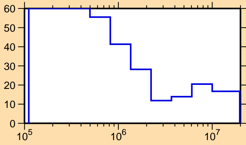
\Delta\sigma/\sigma vs. E for ^{171}\text{Ho}(n,\text{nonel.})
