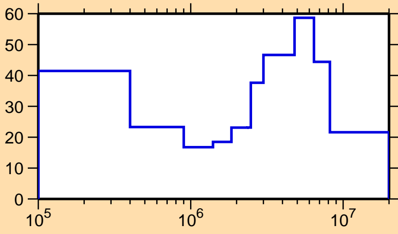
\Delta\sigma/\sigma vs. E for ^{171}\text{Ho}(n, el.)
