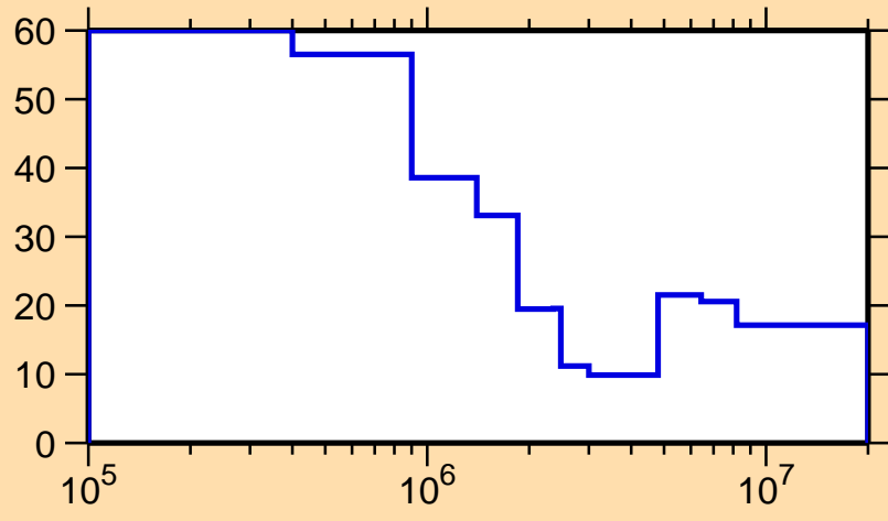
\Delta\sigma/\sigma vs. E for ^{171}\text{Ho}(n,n\text{onel.})
