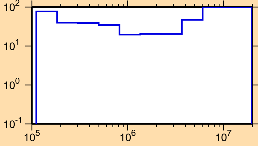
\Delta\sigma/\sigma vs. E for ^{172}\text{Ho}(n,n\text{cont.})
