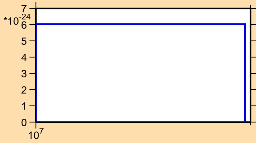
\sigma vs. E for ^{172}\text{Ho} (mt 42)
