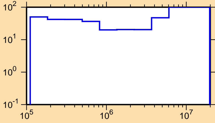
\Delta\sigma/\sigma vs. E for ^{172}\text{Ho}(n,\text{inel.})
