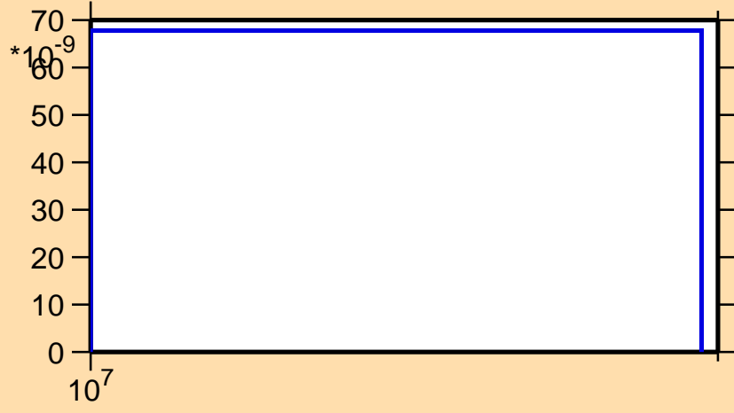
\sigma vs. E for ^{172}\text{Ho}(n,nt)
