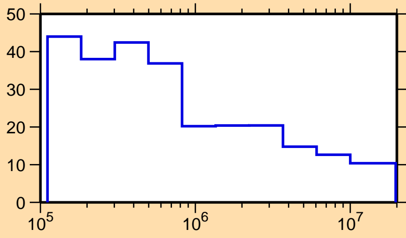
\Delta\sigma/\sigma vs. E for ^{172}\text{Ho}(n,\text{nonel.})
