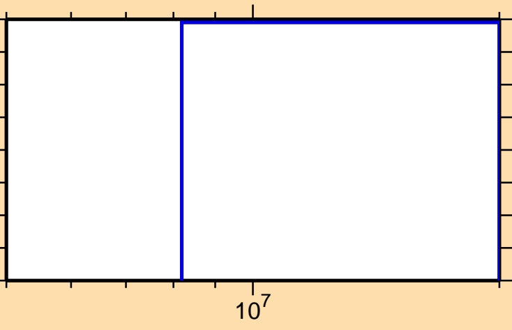
\sigma vs. E for ^{172}\text{Ho}(n,np)
