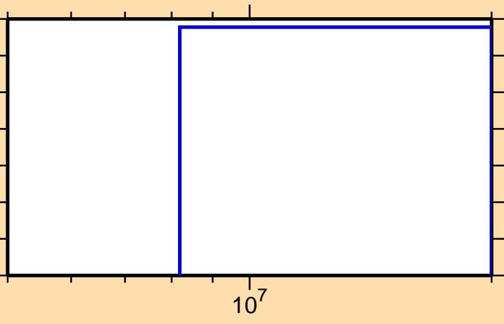
\sigma vs. E for ^{172}\text{Ho}(n,\text{nd})
