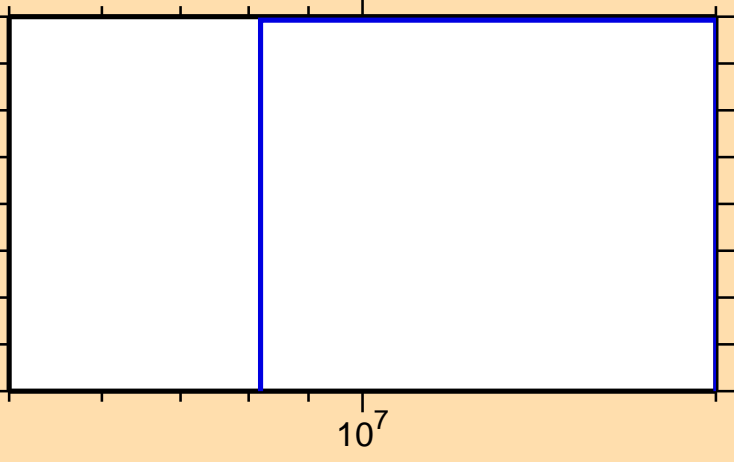
\sigma vs. E for ^{172}\text{Ho}(n,n\alpha)
