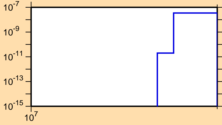
\sigma vs. E for ^{173}\text{Ho}(n,2np)
