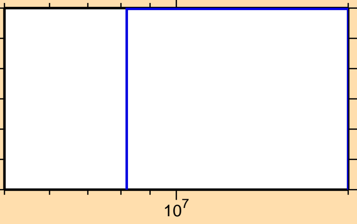
\sigma vs. E for ^{173}\text{Ho}(n,\text{nd})
