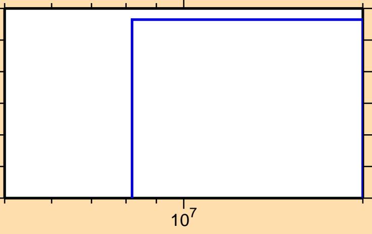
\sigma vs. E for ^{173}\text{Ho}(n,2np)
