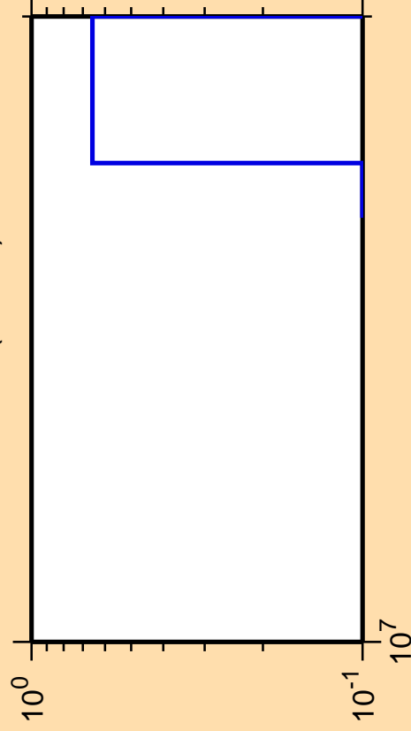
\Delta\sigma/\sigma vs. E for ^{174}\text{Ho} (mt 11)
