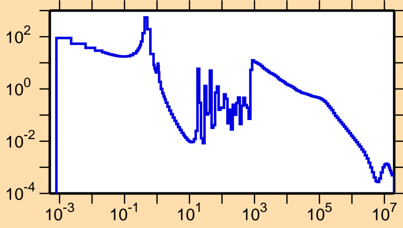
\sigma vs. E for ^{174}\text{Ho}(n,\gamma)
