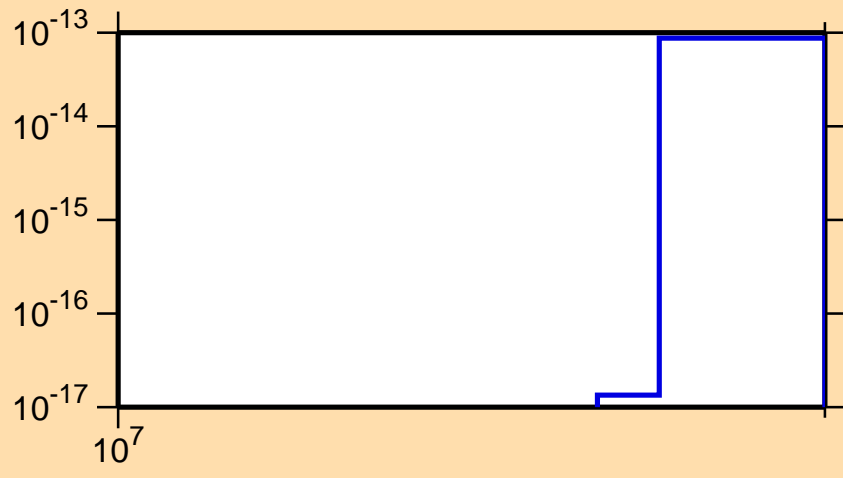
\sigma vs. E for ^{174}\text{Ho}(n,3n\alpha)
