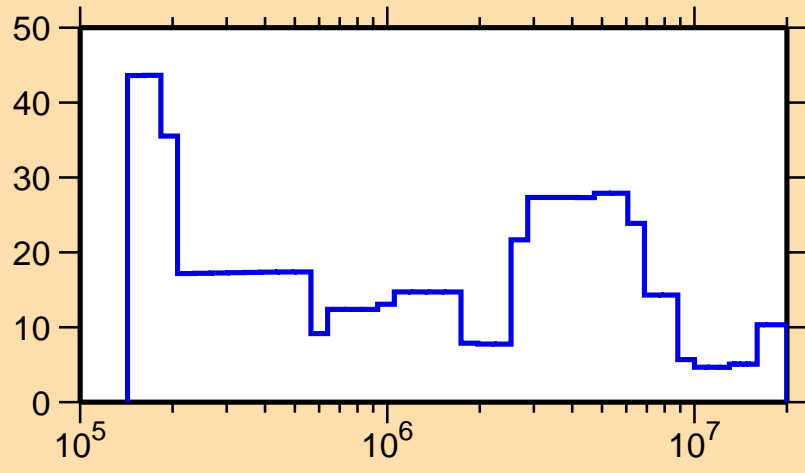
\Delta\sigma/\sigma vs. E for ^{174}\text{Ho}(n,\text{el.})
