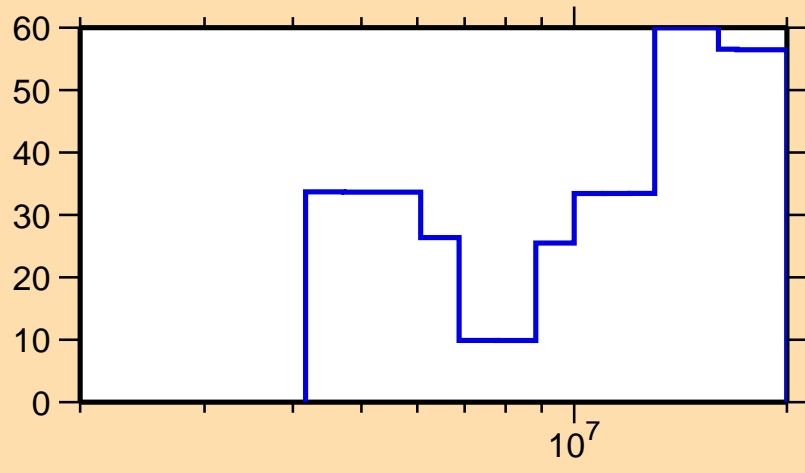
\Delta\sigma/\sigma vs. E for ^{174}\text{Ho}(n,2n)
