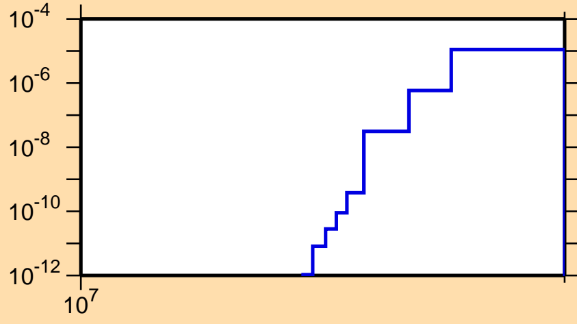
\sigma vs. E for ^{174}\text{Ho}(n,\text{nd})
