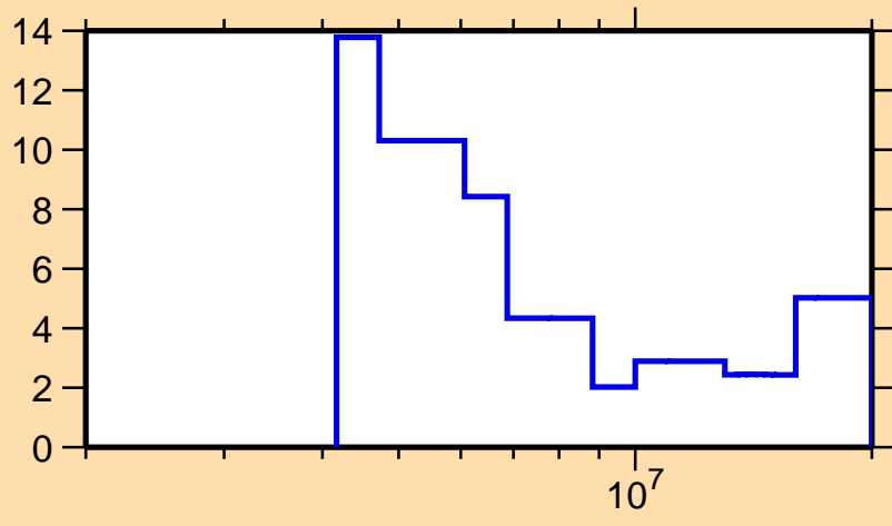
\Delta\sigma/\sigma vs. E for ^{174}\text{Ho}(n,\text{tot.})
