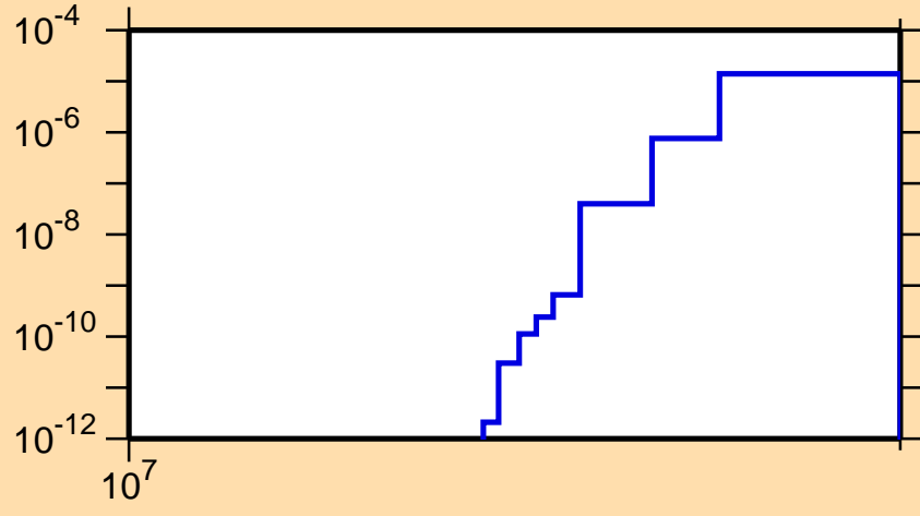
\sigma vs. E for ^{174}\text{Ho}(n,nt)
