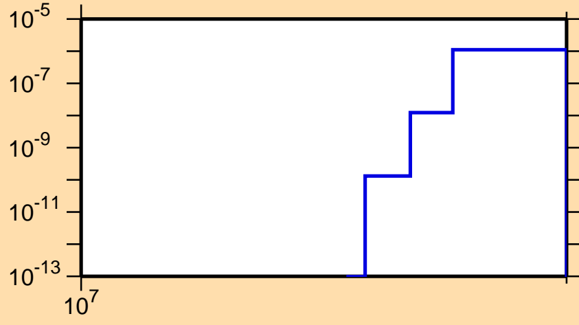
\sigma vs. E for ^{174}\text{Ho}(n,2np)
