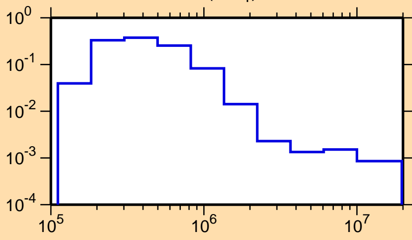
\sigma vs. E for ^{174}\text{Ho}(n,n_1)
