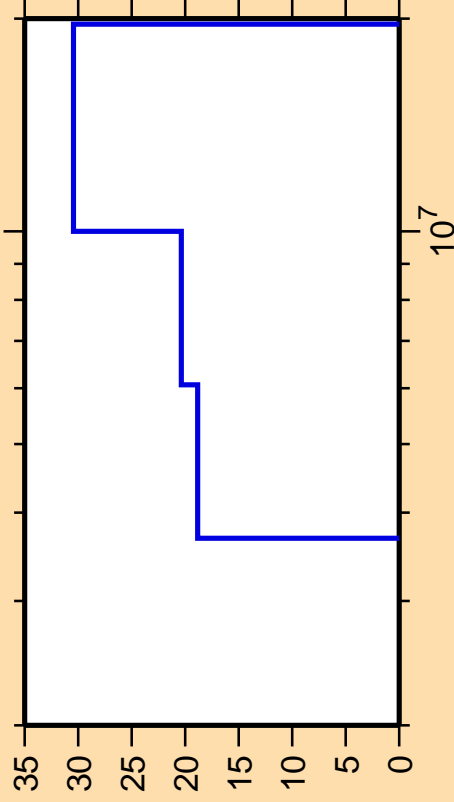
\Delta\sigma/\sigma vs. E for ^{175}\text{Ho}(n,n\text{cont.})
