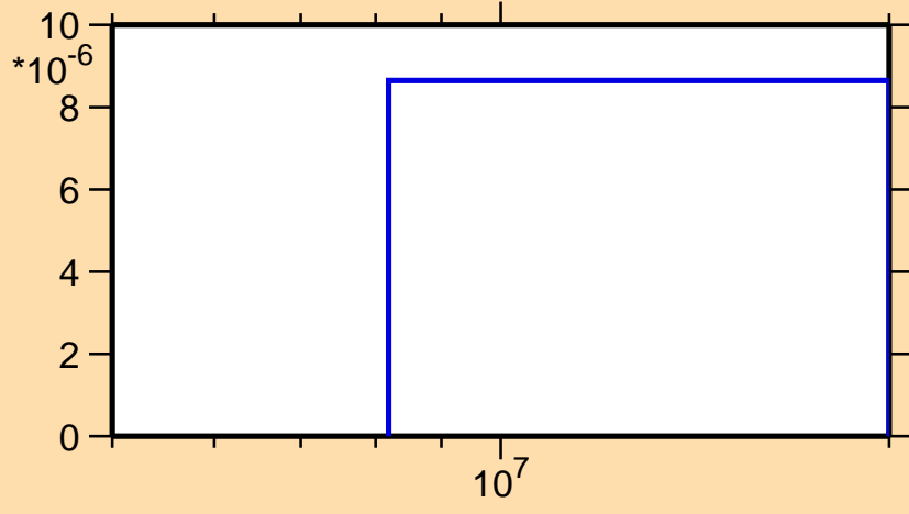
\sigma vs. E for ^{175}\text{Ho}(n,t)
