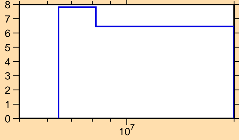
\Delta\sigma/\sigma vs. E for ^{175}\text{Ho}(n,\text{nonel.})
