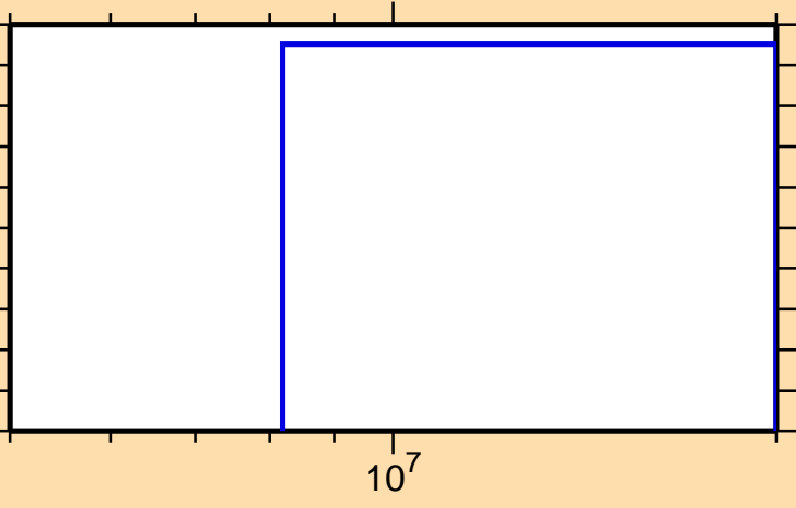
\sigma vs. E for ^{175}\text{Ho}(n,d)
