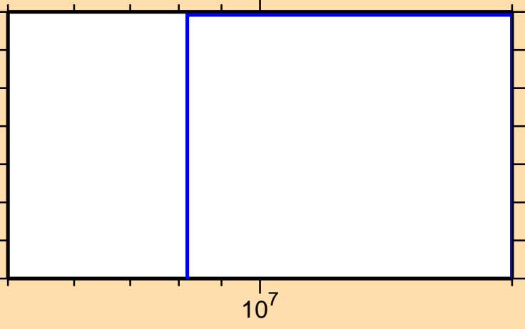
\sigma vs. E for ^{175}\text{Ho}(n,np)
