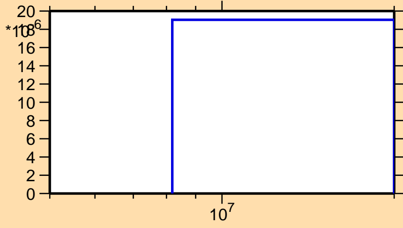
\sigma vs. E for ^{175}\text{Ho}(n,d)
