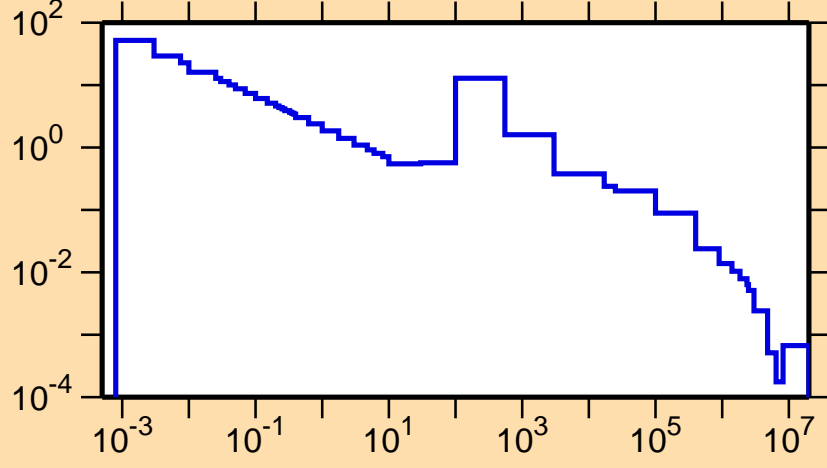
\sigma vs. E for ^{175}\text{Ho}(n,\gamma)
