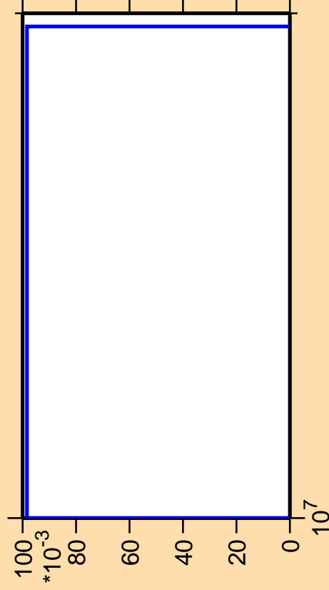
\Delta\sigma/\sigma vs. E for ^{269}
