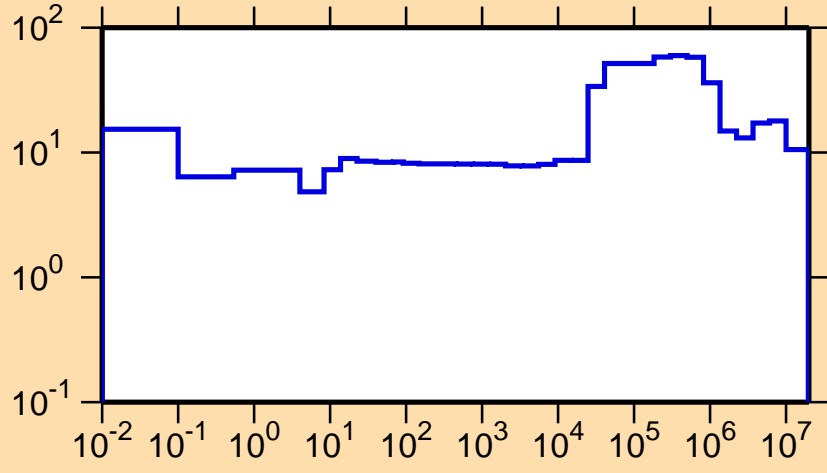
\Delta\sigma/\sigma vs. E for ^{269}\text{Tm}
