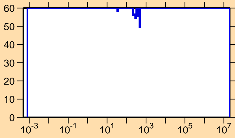
\Delta\sigma/\sigma vs. E for ^{272}\gamma
