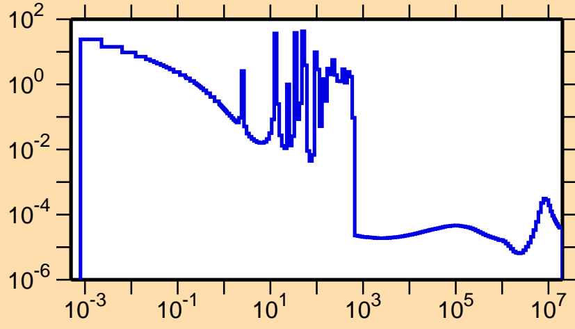
\sigma vs. E for ^{272}\gamma
