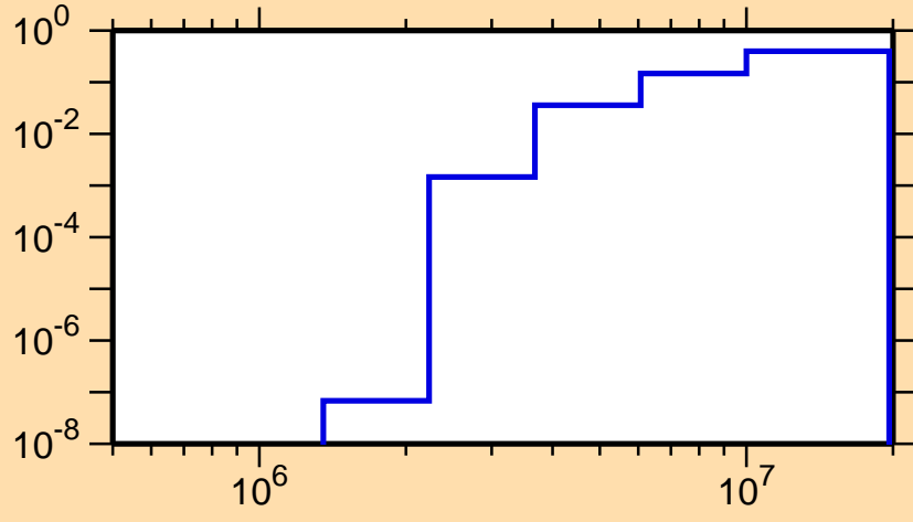
\sigma vs. E for ^{112}\text{I}(n,np)
