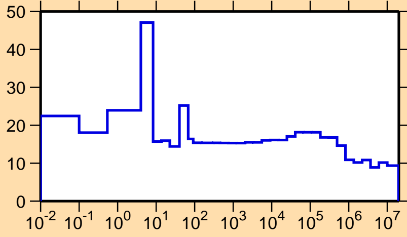
\Delta\sigma/\sigma vs. E for ^{112}\text{I}(n,el.)
