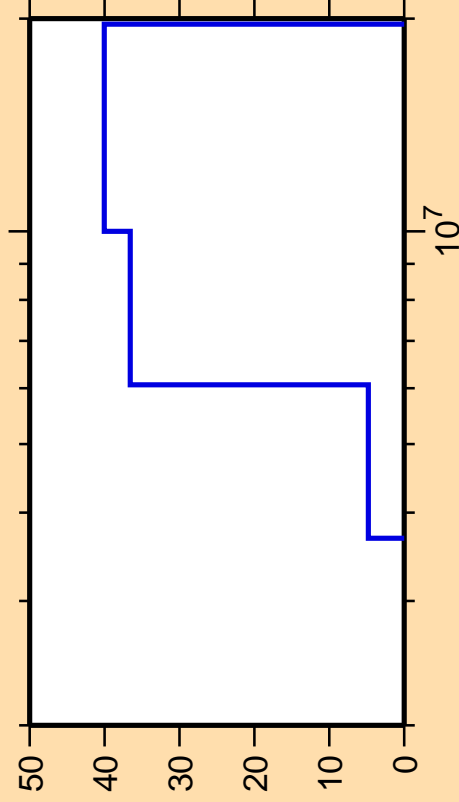
\Delta\sigma/\sigma vs. E for ^{112}\text{I}(\text{mt } 45)
