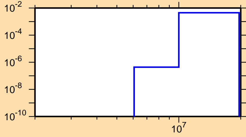
\sigma vs. E for ^{112}\text{I}(\text{mt } 45)
