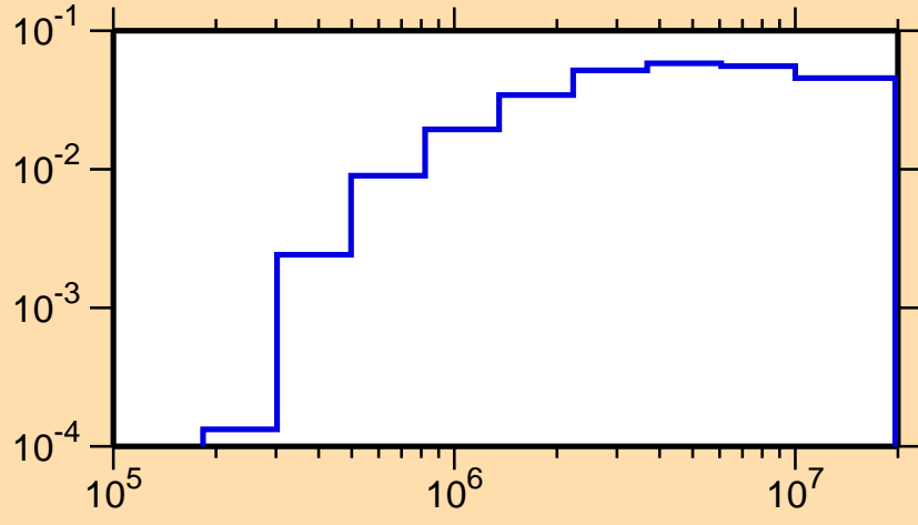
\sigma vs. E for ^{112}\text{I}(n,n\text{cont.})
