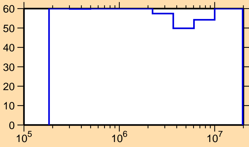
\Delta\sigma/\sigma vs. E for ^{112}\text{I}(n,n_1)
