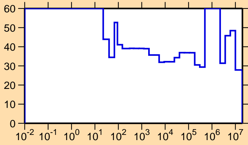
\Delta\sigma/\sigma vs. E for ^{112}\text{I}(n,\gamma)
