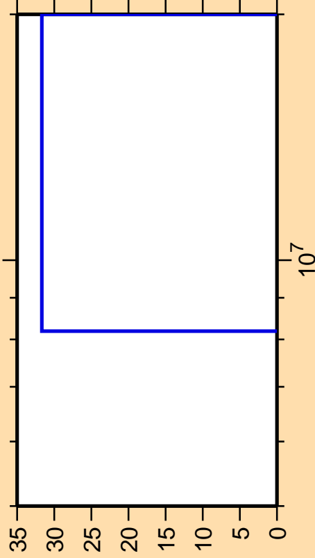
\Delta\sigma/\sigma vs. E for ^{112}\text{I}(n,\gamma)
