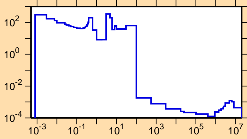
\sigma vs. E for ^{112}\text{I}(n,\gamma)
