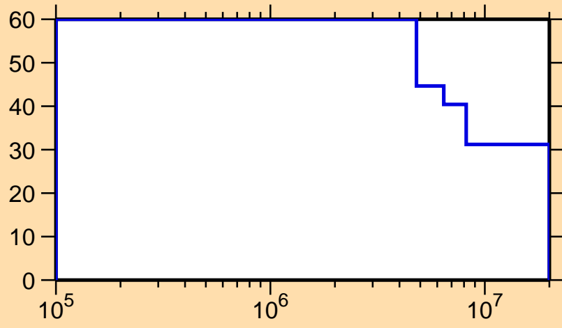
\Delta\sigma/\sigma vs. E for ^{112}\text{I}(n,n\text{cont.})
