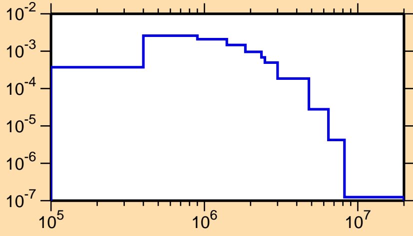
\sigma vs. E for ^{112}\text{I}(n,n_1)
