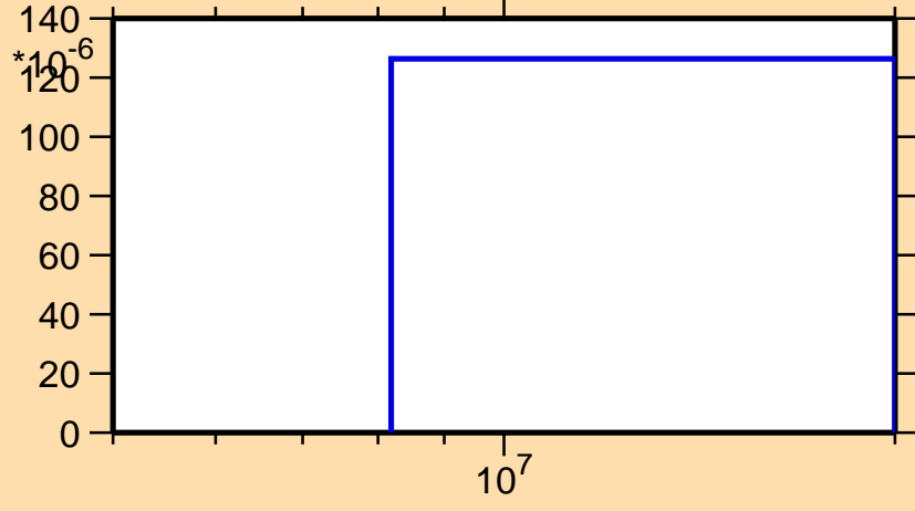
\sigma vs. E for ^{112}\text{I}(n,2np)
