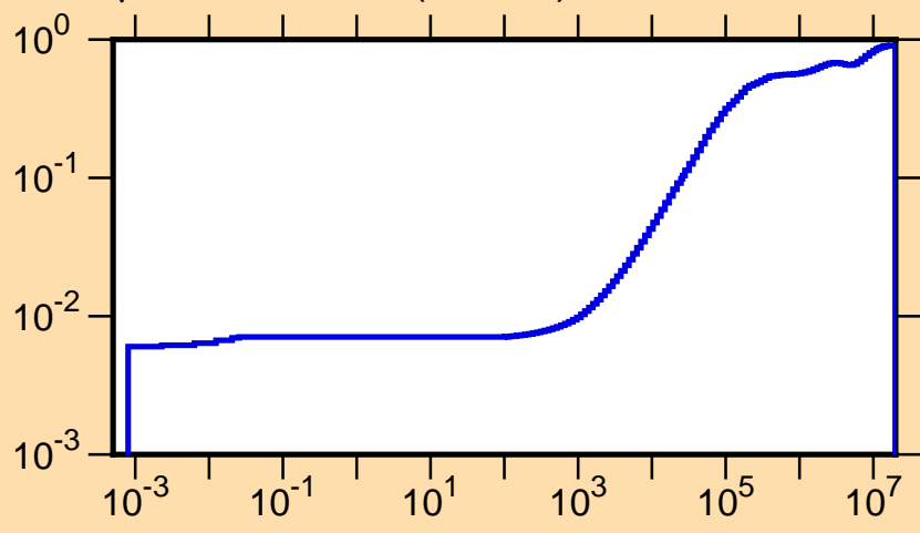
\mu vs. E for ^{113}\text{I}(\text{mt251})
