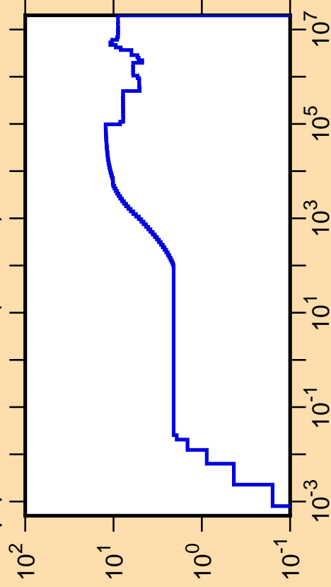
\Delta\mu/\mu vs. E for ^{113}\text{I}(\text{mt251})
