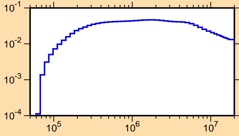
\sigma vs. E for ^{113}\text{I}(n,n_1)
