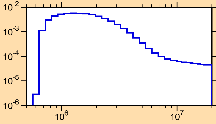
\sigma vs. E for ^{113}\text{I}(n,n_2)
