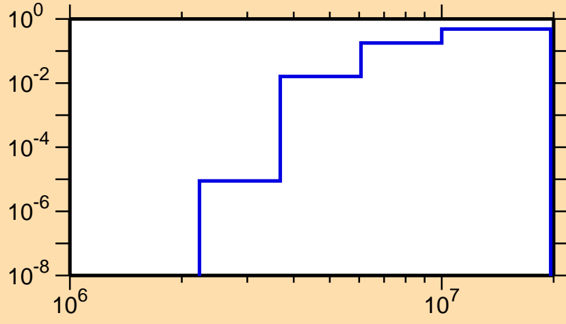
\sigma vs. E for ^{113}\text{I}(n,np)
