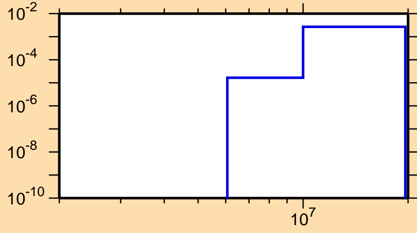
\sigma vs. E for ^{113}\text{I} (mt 45)
