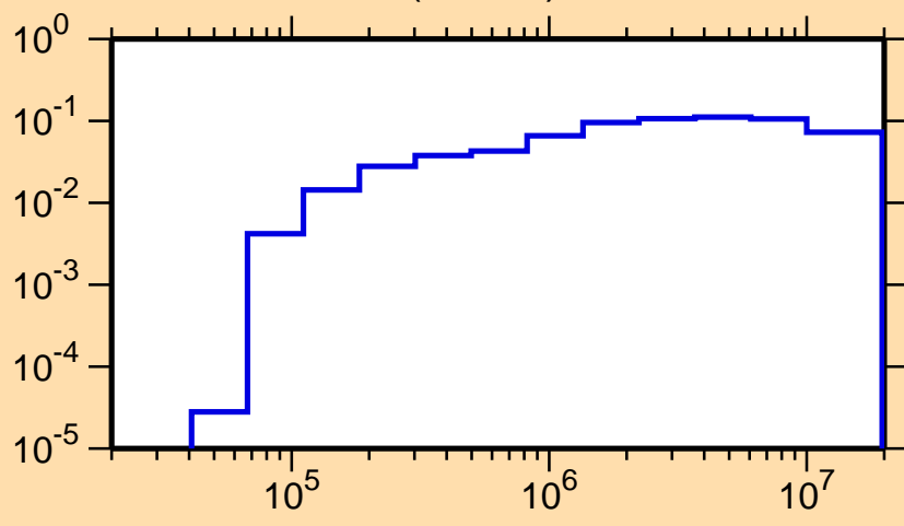
\sigma vs. E for ^{113}\text{I}(n,\text{inel.})
