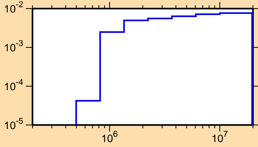
\sigma vs. E for ^{113}\text{I}(n,n_3)
