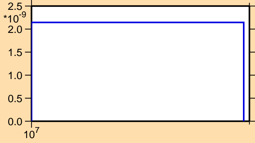
\sigma vs. E for ^{113}\text{I}(n,2n\alpha)
