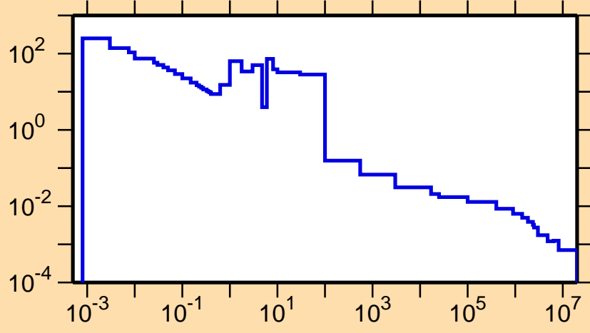
\sigma vs. E for ^{113}\text{I}(n,\gamma)
