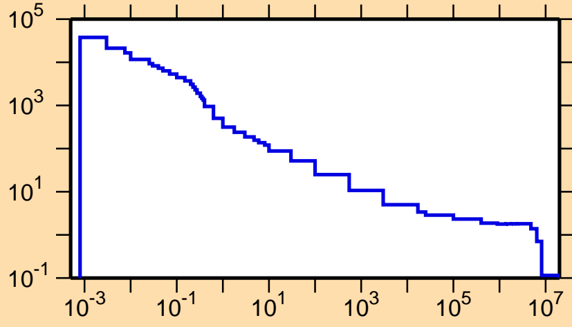
\sigma vs. E for ^{113}\text{I}(n,p)
