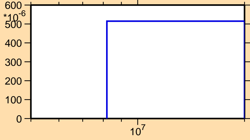
\sigma vs. E for ^{113}\text{I}(n,2n)
