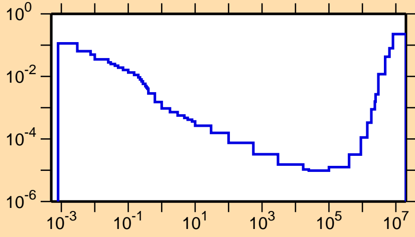
\sigma vs. E for ^{113}\text{I}(n,p\alpha)
