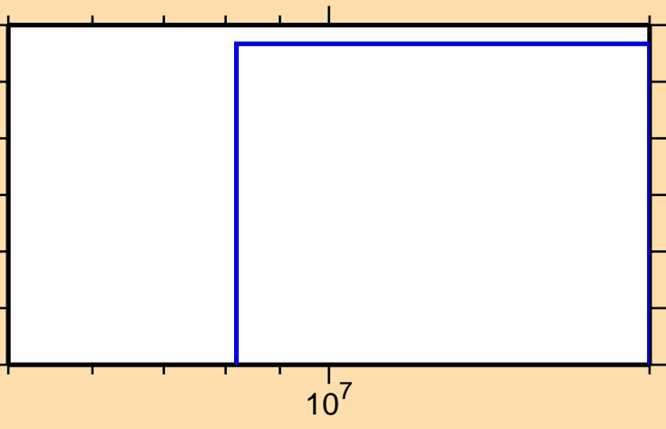
\sigma vs. E for ^{113}\text{I}(n,2np)
