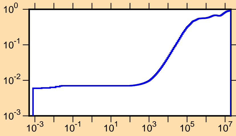
\mu vs. E for ^{114}\text{I}(\text{mt251})
