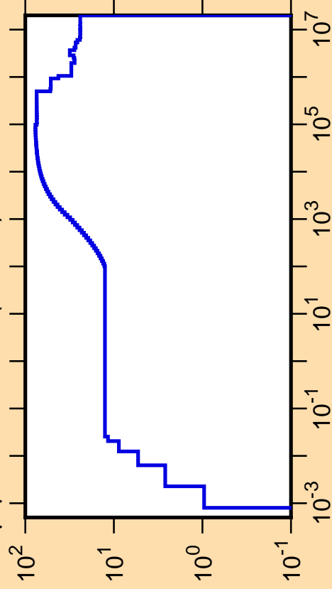
\Delta\mu/\mu vs. E for ^{114}\text{I}(\text{mt251})
