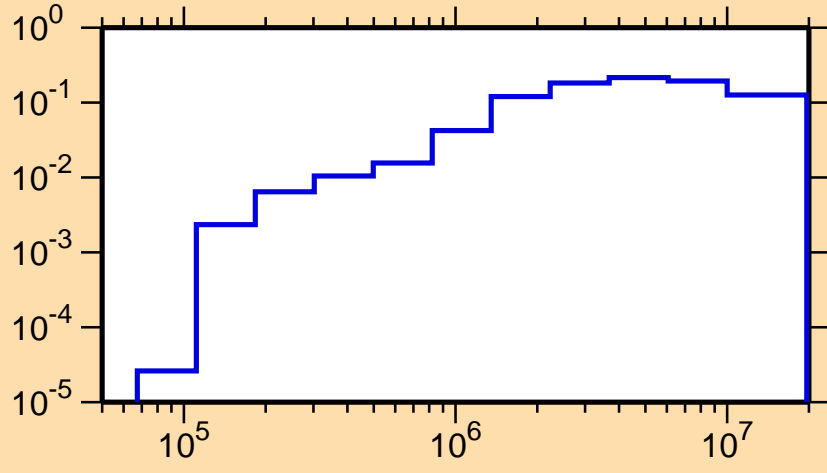
\sigma vs. E for ^{114}\text{I}(n,\text{inel.})
