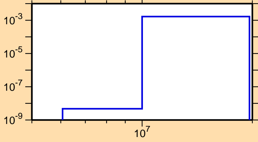
\sigma vs. E for ^{114}\text{I}(\text{mt } 45)
