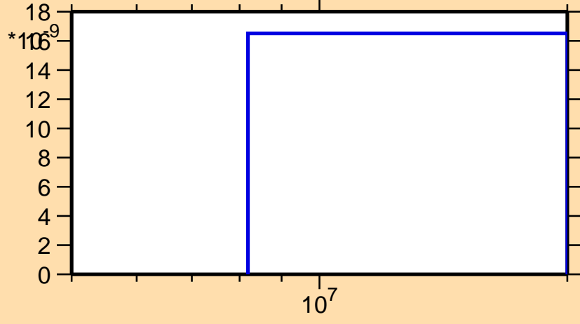
\sigma vs. E for ^{114}\text{I}(\text{mt } 34)
