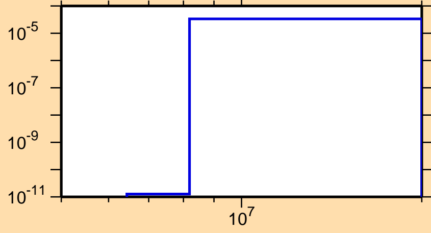
\sigma vs. E for ^{114}\text{I}(\text{mt117})
