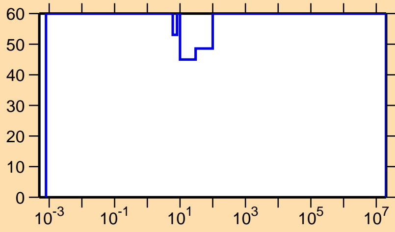
\Delta\sigma/\sigma vs. E for ^{114}\text{I}(n,\gamma)
