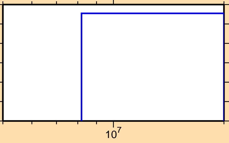
\sigma vs. E for ^{114}\text{I}(n,\text{nd})
