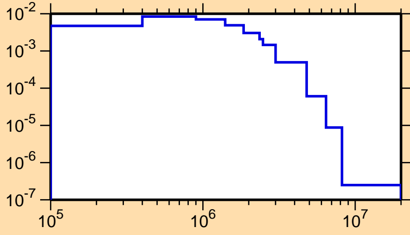
\sigma vs. E for ^{114}\text{I}(n,n_1)
