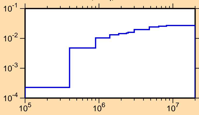
\sigma vs. E for ^{114}\text{I}(n,n_4)
