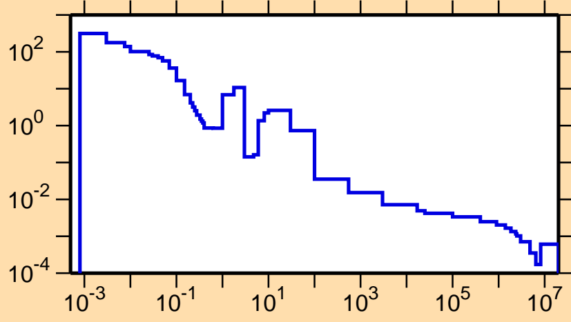
\sigma vs. E for ^{114}\text{I}(n,\gamma)
