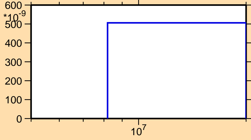
\sigma vs. E for ^{114}\text{I}(n,2n\alpha)
