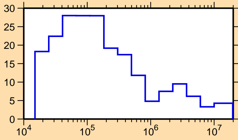
\Delta\sigma/\sigma vs. E for ^{114}\text{I}(n, tot.)
