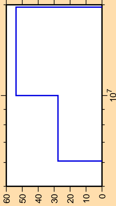
\Delta\sigma/\sigma vs. E for ^{114}\text{I}(n,n_1)
