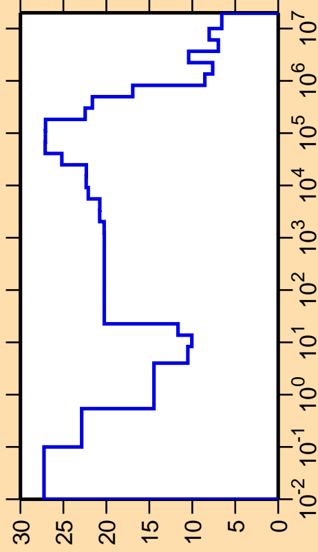
\Delta\sigma/\sigma vs. E for ^{114}\text{I}(n,\text{el.})
