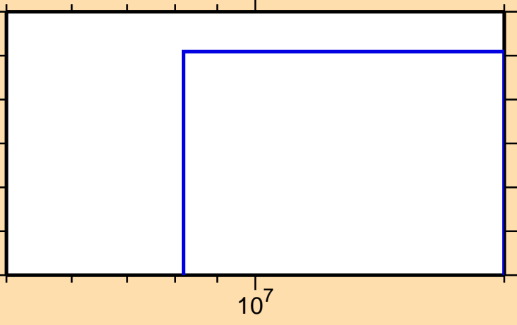
\sigma vs. E for ^{114}\text{I}(n,2n)
