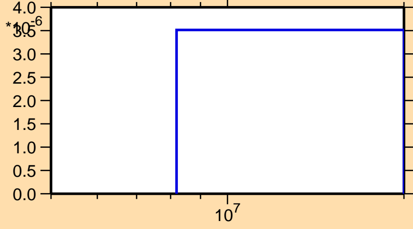
\sigma vs. E for ^{114}\text{I}(n,\text{nd})
