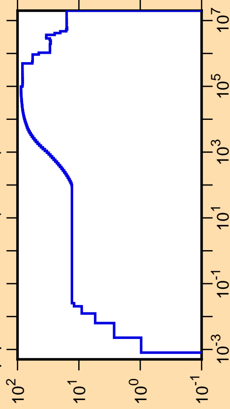
\Delta\mu/\mu vs. E for ^{115}\text{I} (mt251)
