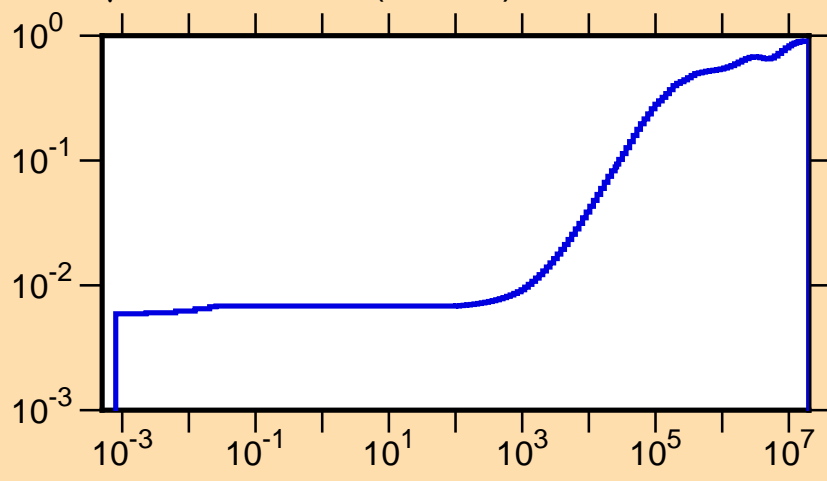
\mu vs. E for ^{115}\text{I} (mt251)
