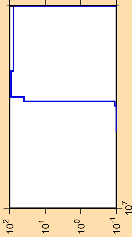
\Delta\sigma/\sigma vs. E for ^{115}\text{I}(n,2np)
