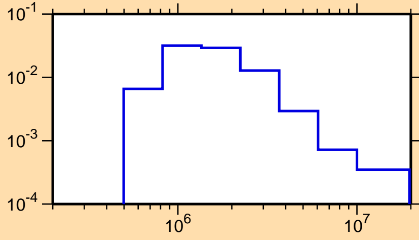
\sigma vs. E for ^{115}\text{I}(n,n_3)
