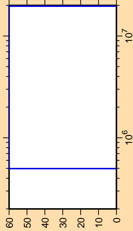
\Delta\sigma/\sigma vs. E for ^{115}\text{I}(n,n_3)
