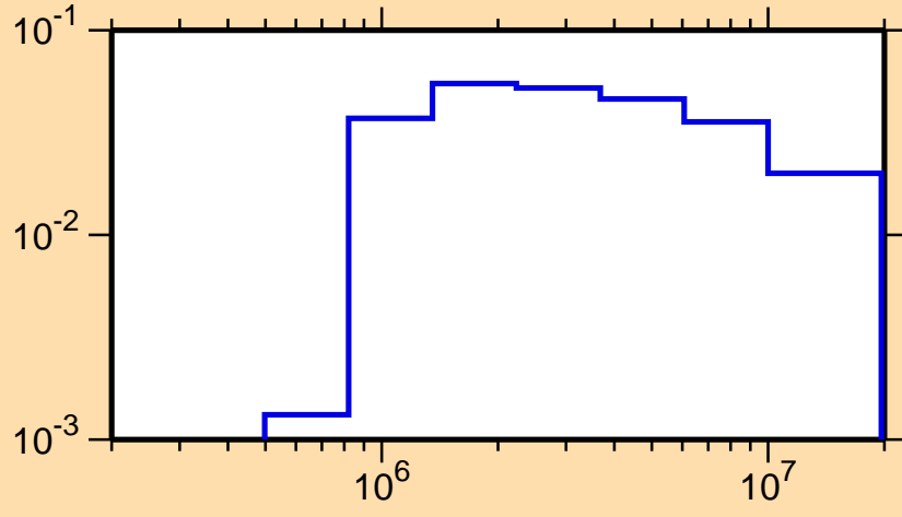
\sigma vs. E for ^{115}\text{I}(n,n_4)
