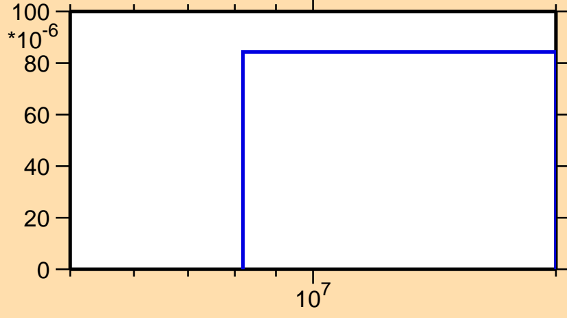
\sigma vs. E for ^{115}\text{I}(n,\text{pd})
