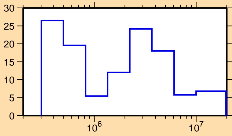
\Delta\sigma/\sigma vs. E for ^{116}\text{I}(n, el.)
