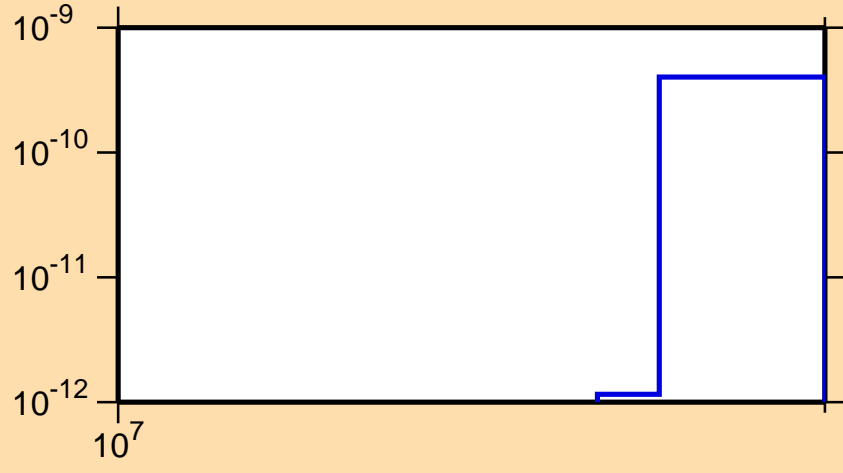
\sigma vs. E for ^{117}\text{I} (mt 34)
