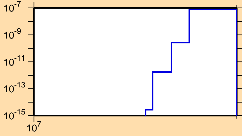
\sigma vs. E for ^{117}\text{I}(n,\text{pt})
