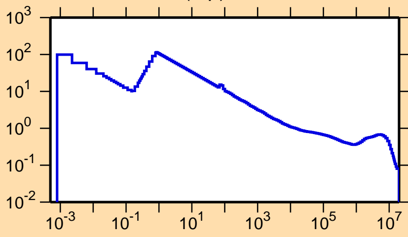
\sigma vs. E for ^{117}\text{I}(n,p)
