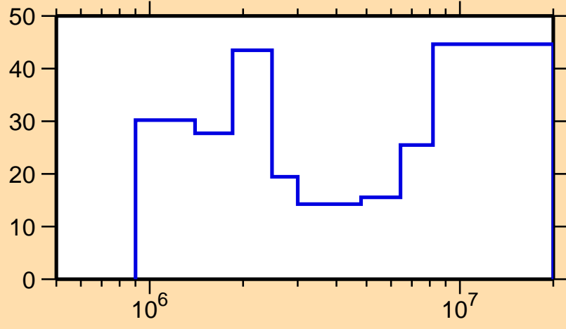
\Delta\sigma/\sigma vs. E for ^{117}\text{I}(n,n\text{cont.})
