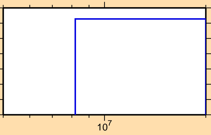
\sigma vs. E for ^{117}\text{I}(n,2np)
