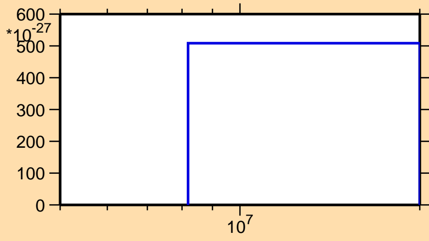
\sigma vs. E for ^{117}\text{I} (mt 11)
