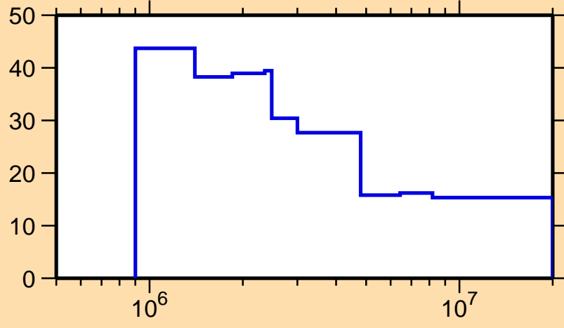
\Delta\sigma/\sigma vs. E for ^{117}\text{I}(n,n_1)
