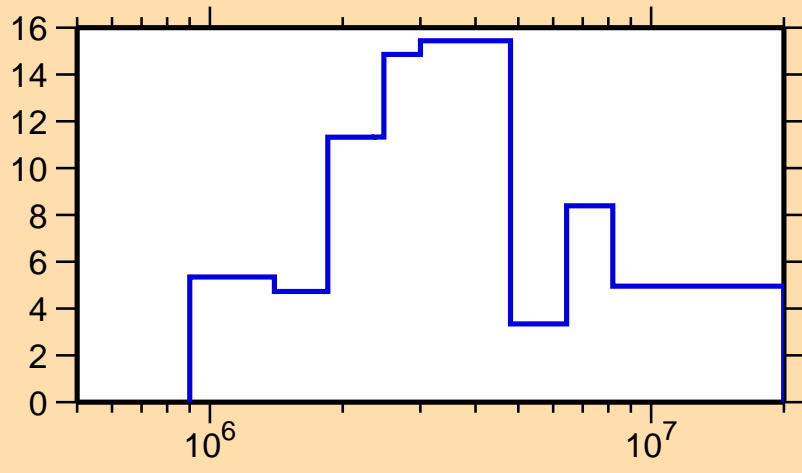
\Delta\sigma/\sigma vs. E for ^{117}\text{I}(n, el.)
