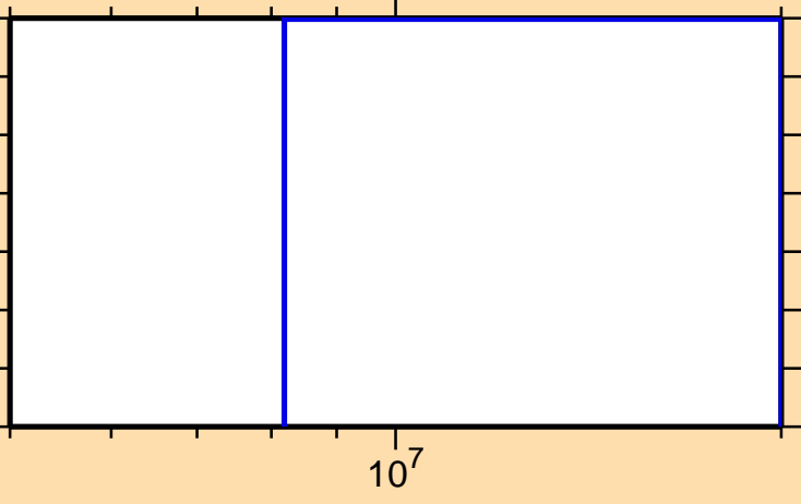
\sigma vs. E for ^{118}\text{I}(n,3n)
