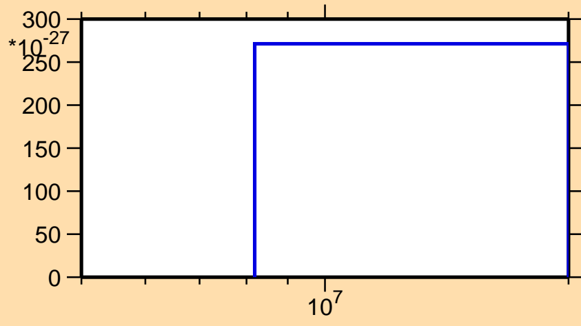
\sigma vs. E for ^{118}\text{I}(\text{mt 11})
