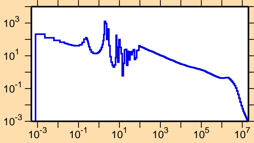
\sigma vs. E for ^{119}\text{I}(n,\gamma)
