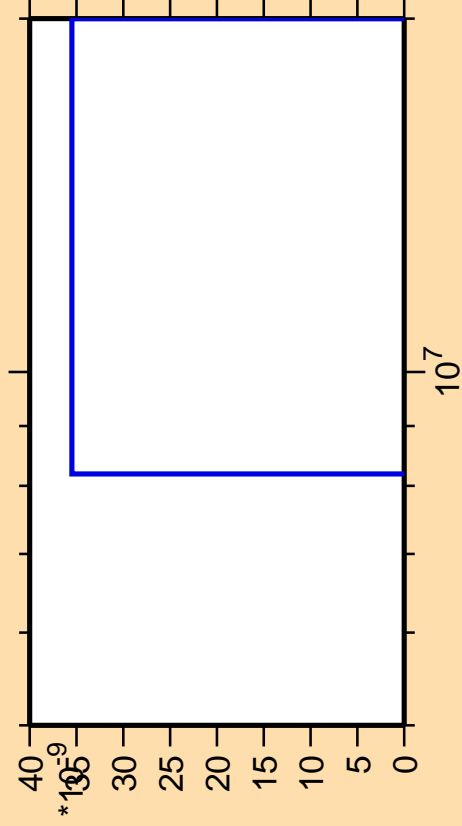
\Delta\sigma/\sigma vs. E for ^{119}\text{I}(n,3n\alpha)
