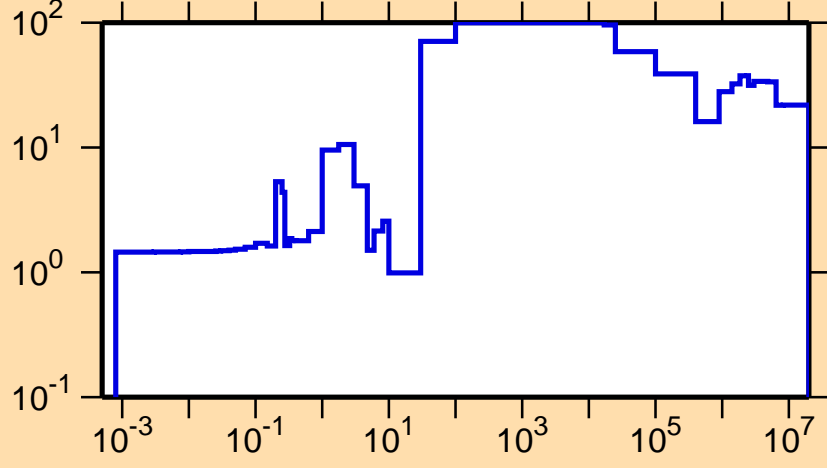
\Delta\sigma/\sigma vs. E for ^{119}\text{I}(n,el.)
