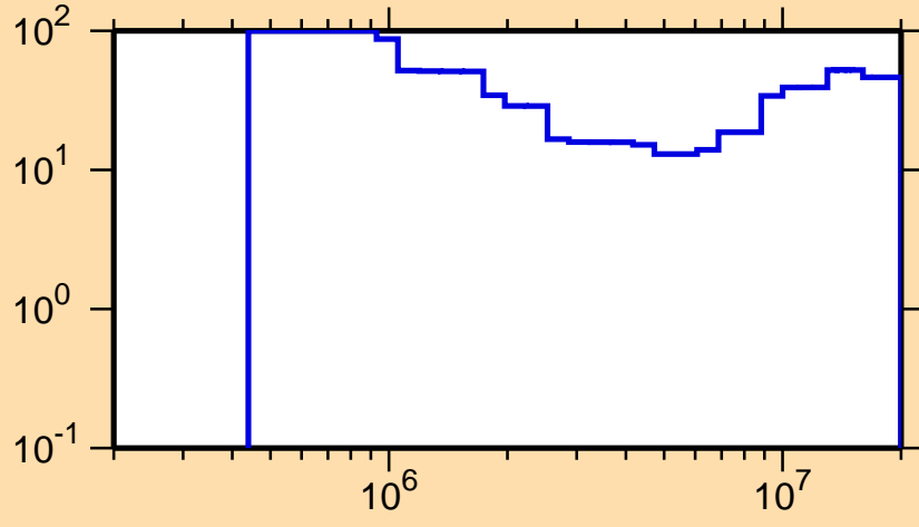
\Delta\sigma/\sigma vs. E for ^{120}\text{I}(n,n\text{cont.})
