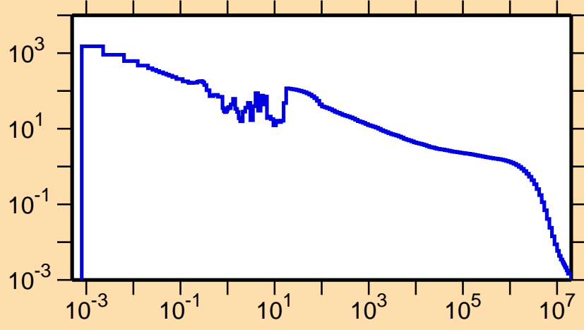
\sigma vs. E for ^{120}\text{I}(n,\gamma)
