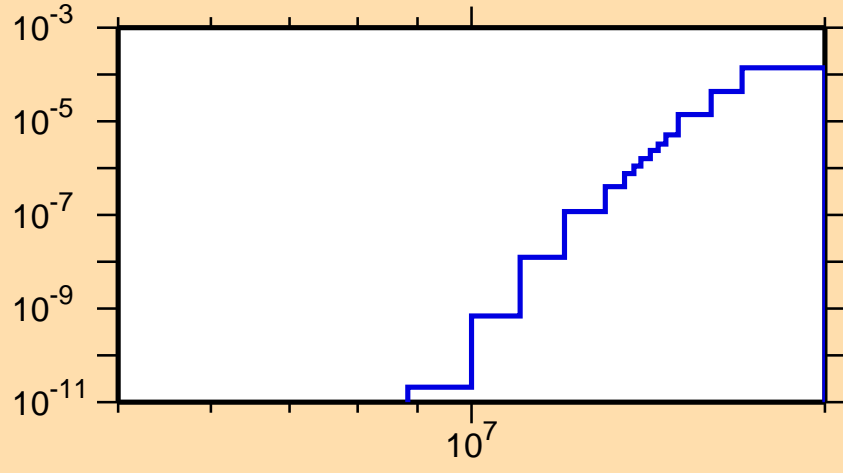
\sigma vs. E for ^{120}\text{I}(n,\text{He3})
