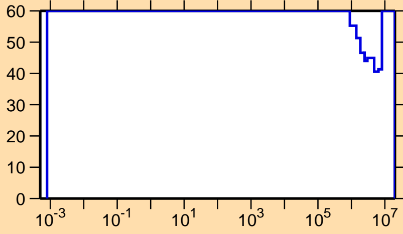
\Delta\sigma/\sigma vs. E for ^{120}\text{I}(n,p)
