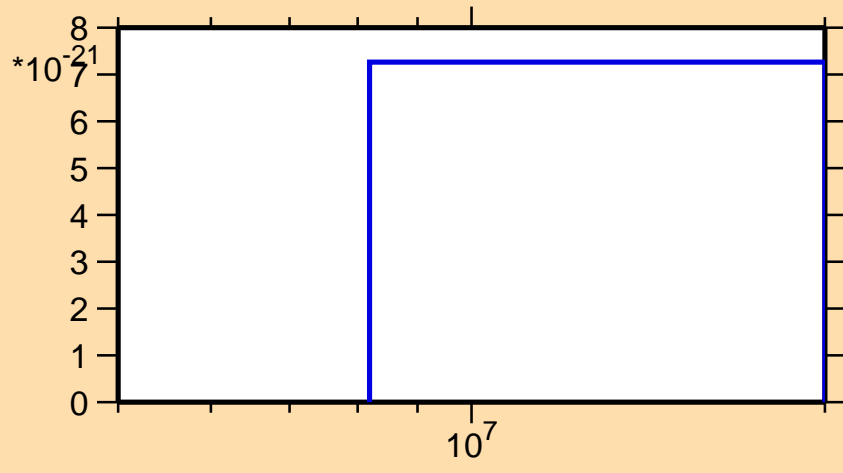
\sigma vs. E for ^{120}\text{I}(\text{mt 11})
