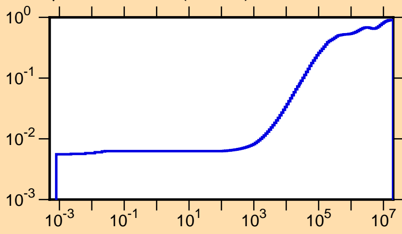
\mu vs. E for ^{122}\text{I}(\text{mt251})
