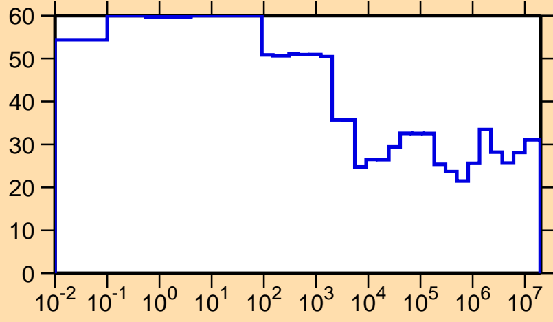
\Delta\sigma/\sigma vs. E for ^{122}\text{I}(n,p)
