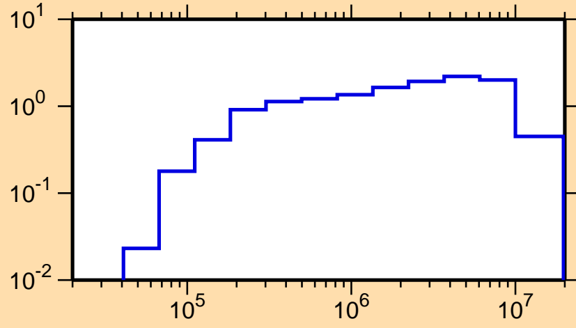
\sigma vs. E for ^{122}\text{I}(n,\text{inel.})
