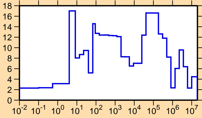
\Delta\sigma/\sigma vs. E for ^{122}\text{I}(n,el.)
