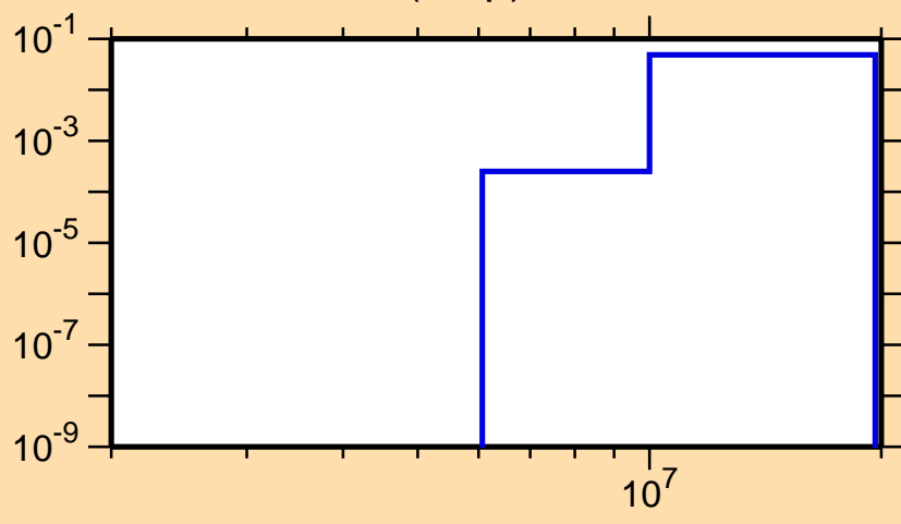
\sigma vs. E for ^{122}\text{I}(n,np)
