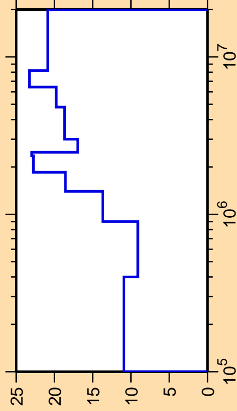
\Delta\sigma/\sigma vs. E for ^{122}\text{I}(n,n_4)
