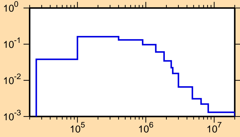
\sigma vs. E for ^{122}\text{I}(n,n_1)
