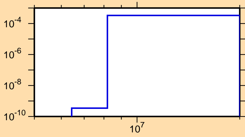
\sigma vs. E for ^{122}\text{I}(n,t)
