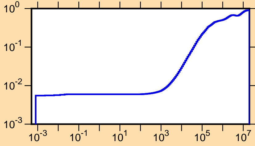
\mu vs. E for ^{123}\text{I} (mt251)
