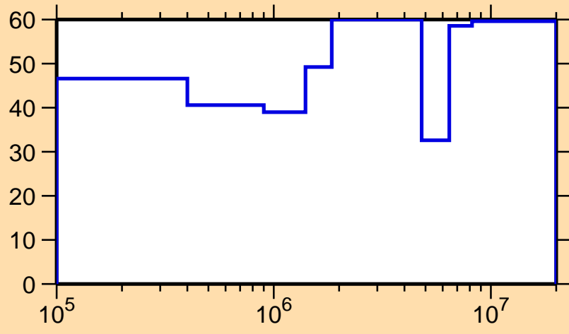
\Delta\sigma/\sigma vs. E for ^{123}\text{I}(n,n_1)
