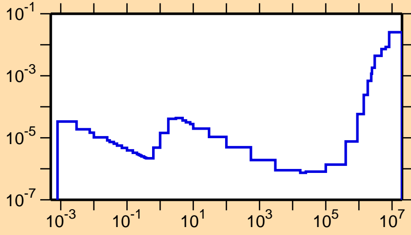
\sigma vs. E for ^{123}\text{I}(n,p)
