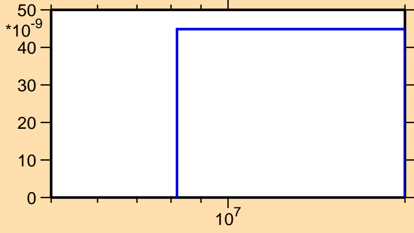
\sigma vs. E for ^{123}\text{I}(n,p\alpha)
