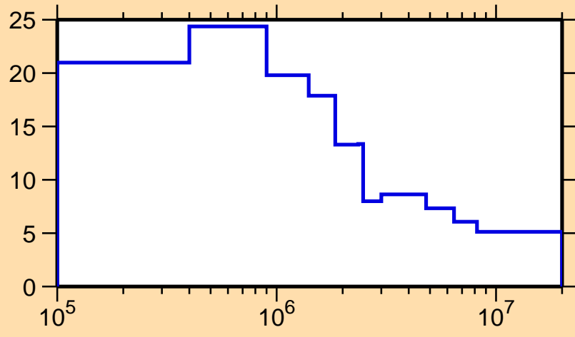
\Delta\sigma/\sigma vs. E for ^{123}\text{I}(n,\text{nonel.})
