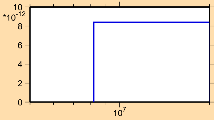
\sigma vs. E for ^{123}\text{I} (mt 45)
