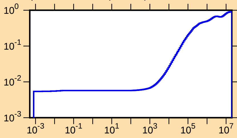
\mu vs. E for ^{125}\text{I}(\text{mt251})
