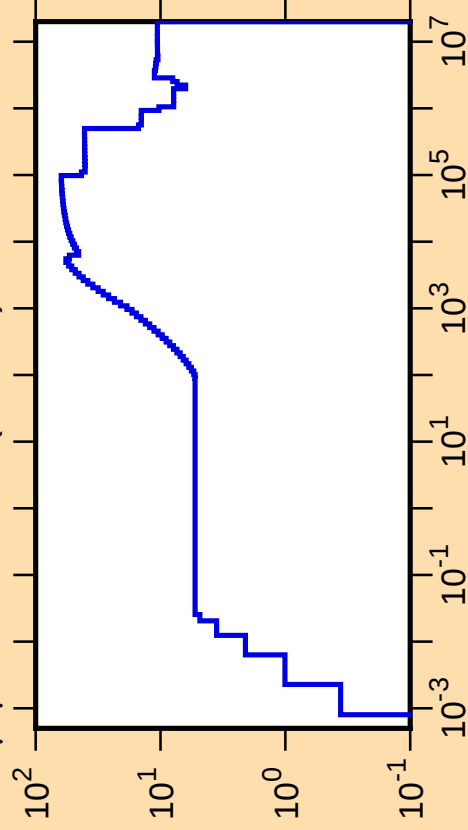
\Delta\mu/\mu vs. E for ^{125}\text{I}(\text{mt251})
