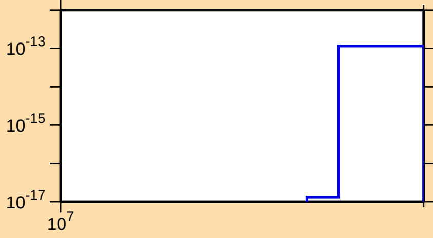
\sigma vs. E for ^{125}\text{I}(\text{n},\text{pd})
