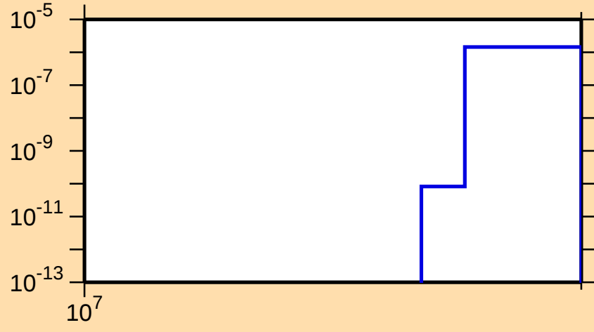
\sigma vs. E for ^{125}\text{I}(n,2np)
