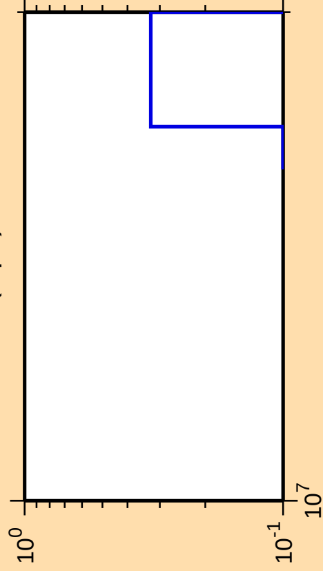
\Delta\sigma/\sigma vs. E for ^{125}\text{I}(\text{n},\text{pd})
